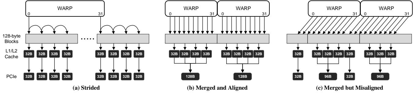
Figure 3: GPU PCIe memory request patterns observed with FPGA. In (a), each thread scans a different 128-byte block and end up making multiple 32B PCIe memory read requests. In (b), individual 32B memory read requests in a contiguous address space occur at the same time and GPU merges them into a single 128B PCIe memory read request. In (c) each warp is performing a misaligned memory request (off by 32B from 128B boundary) resulting in generating a 32B PCIe and 96B PCIe request. In this figure, we assume each memory access is for 4B.
