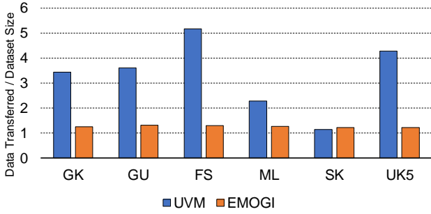
Figure 10: I/O Read Amplification of EMOGI and the UVM baseline while performing BFS. EMOGI has far less I/O read amplification when the graph sizes are significantly larger than the GPU memory.
