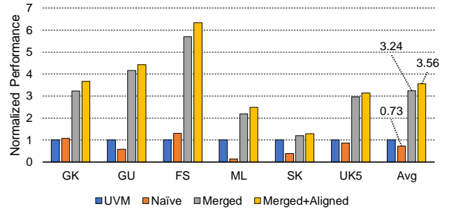
Figure 9: BFS performance of the Naïve, Merged and Merged+Aligned implementations against the UVM baseline. EMOGI’s Merged+Aligned implementation provides the best performance across all graphs.
