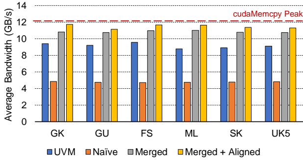
Figure 8: Average PCIe 3.0 x16 bandwidth utilization of the different implementations executing BFS. The Merged+Aligned implementation can nearly saturate the available PCIe bandwidth.
