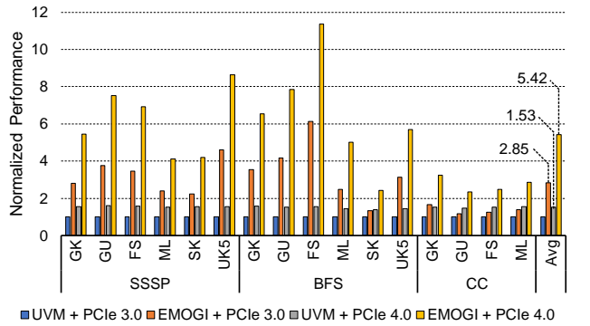
Figure 12: Performance comparison between UVM and EMOGI using PCIe 3.0 and PCIe 4.0. All results are measured in DGX A100. EMOGI is able to scale almost linearly with the PCIe bandwidth.
